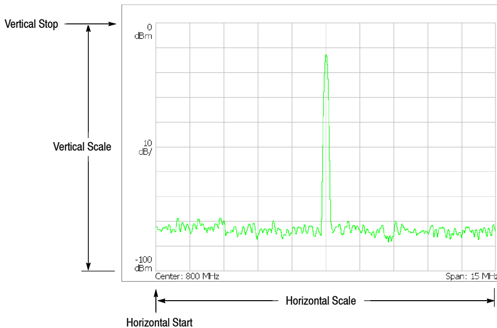
Figure 3- 128: Setting the scale in spectrum view
