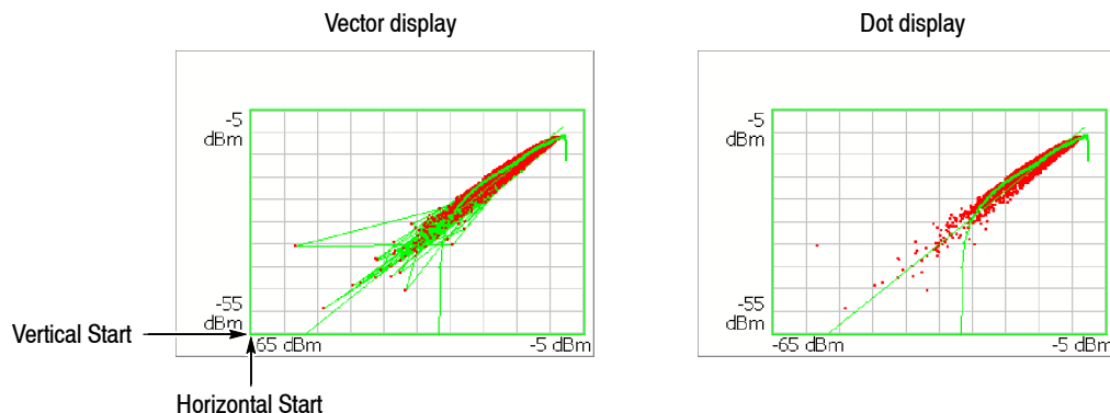
Figure 3-138: Vector and dot displays for AM/AM view
