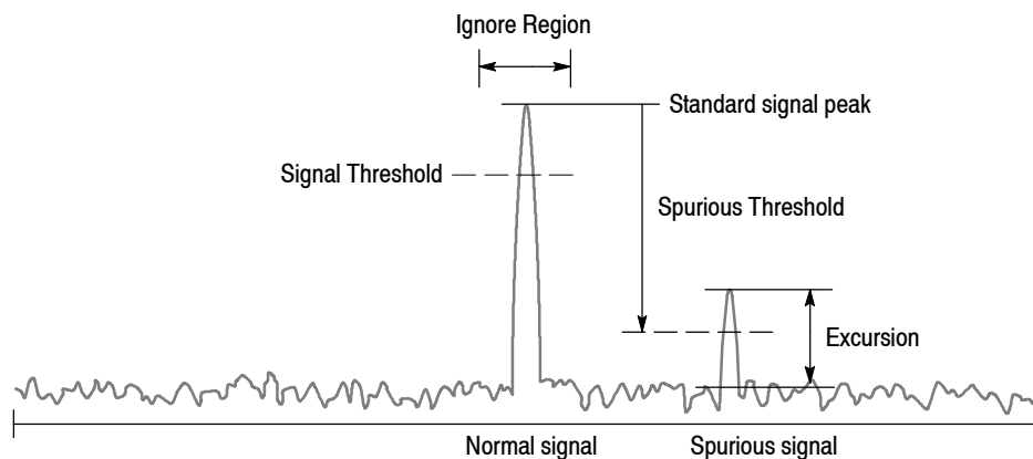
Figure 3-15: Setting up spurious signal measurement
