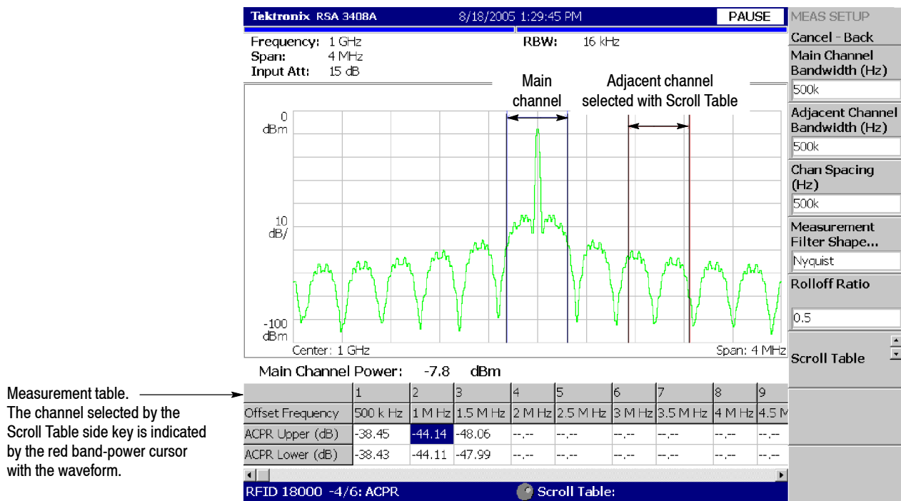
Figure 3-54: ACPR measurements
